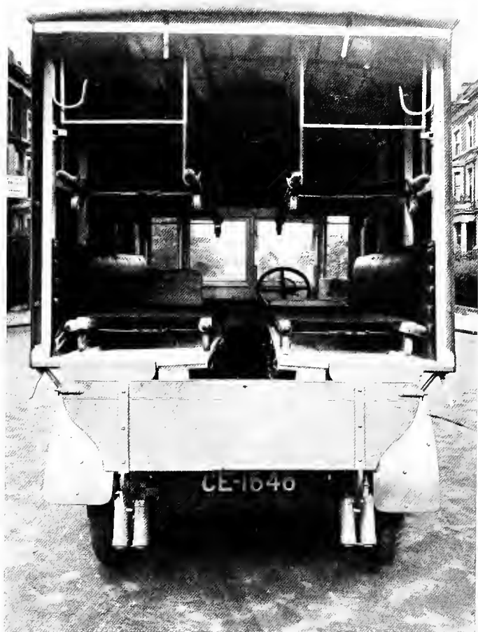
Interior of the new type St. John ambulance, a side view of which is shown in another illustration.
