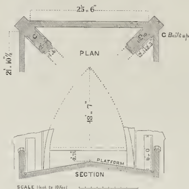
THE PLAN OF THE CROWN STEEPLE, KING'S COLLEGE, ABERDEEN.
